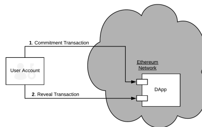
Fig. 8: Commit and Reveal. User sends a commitment transaction with the hash of the data, After the commitment period is over, user sends her reveal transaction to the DApp revealing the information that matches the commitment.
