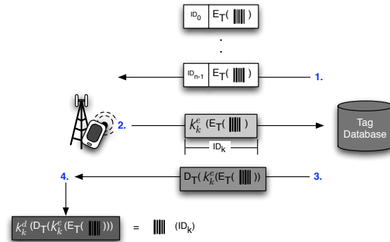
Fig. 2. A 1-out-of- n oblivious transfer as used in ShopAnon. The client 1) receives n encrypted barcodes from the Tag Database. Using the prepended identifier, the client determines which tag it would like to receive, 2) removes the identifier, encrypts the tag with its key (modular multiplication with random k ) and returns it to the tag database. The Tag Database then 3) decrypts the received tag, and sends the resulting ciphertext to the client. Finally, 4) the client decrypts the received ciphertext (modular division by k ) and recovers the desired barcode. Note that the Tag Database can not determine the identity of the tag selected by the client because it can not fully decrypt any of the ciphertexts.
