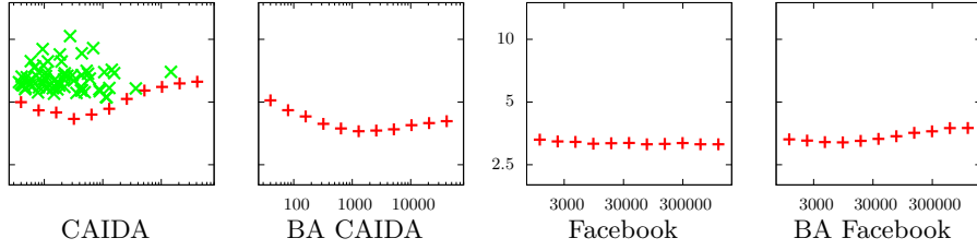
Fig. 6. Ratio of safety loading (for 0.999) to standard deviation for random samples (red +) and countries (green x).
