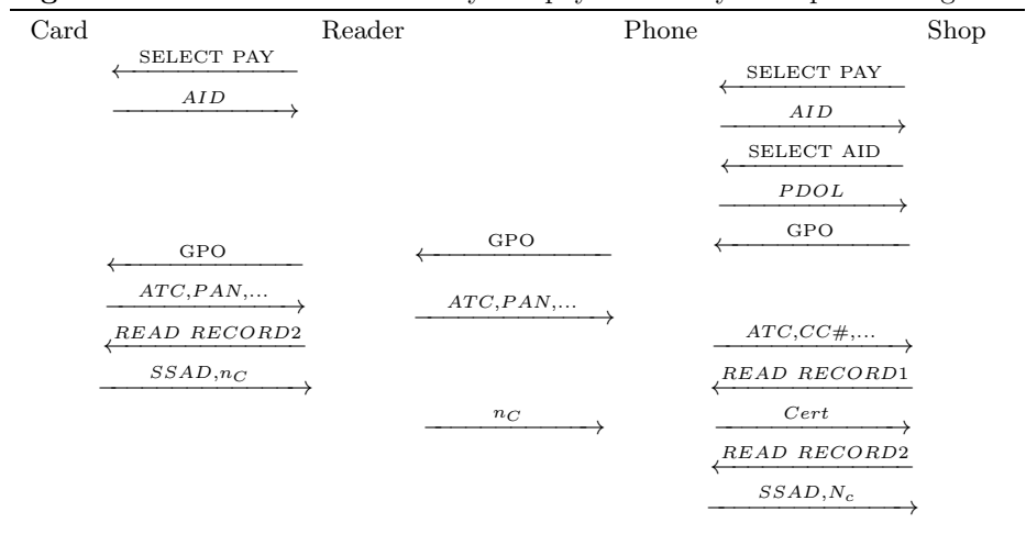
Fig. 3 The communications made by our payWave relay after pre-caching
