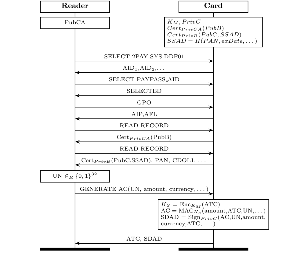
Fig. 1 The PayPass Protocol
